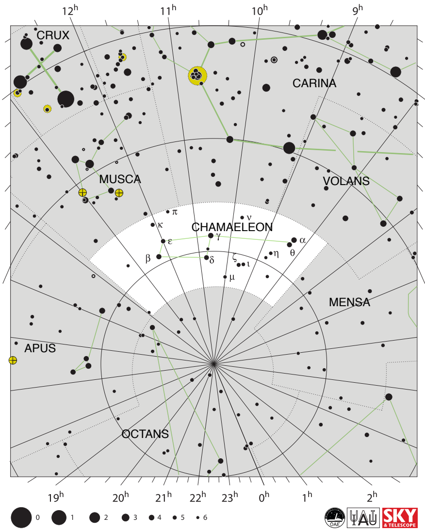
Adapted by the IAU Office of Astronomy for Education from the original by the IAU and Sky & Telescope
