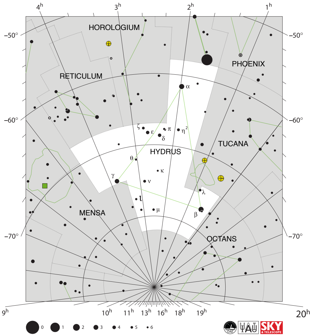
Adapted by the IAU Office of Astronomy for Education from the original by the IAU and Sky & Telescope
